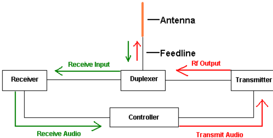
BASIC REPEATER BLOCK DIAGRAM
